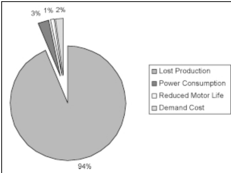
Figure 1: 100 Horsepower Main Drive, 5% Impedance Unbalance
