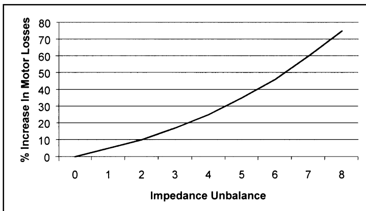
Figure 5: Increase in Losses Due to Impedance Unbalance
