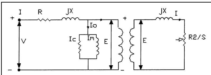
Figure 2: One Phase of An Electric Motor Circuit
