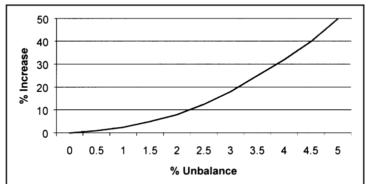
Figure 6: Increase in Temperature Rise Due to Impedance Unbalance
