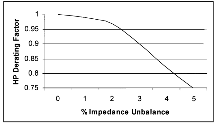
Figure 4: Horsepower Derating Factor Due to Impedance Unbalance
