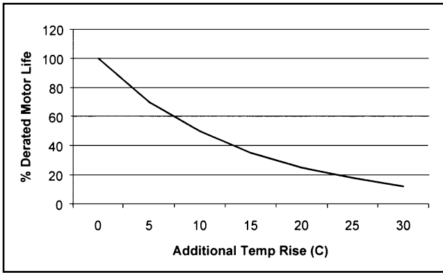
Figure 7: Reduced Reliability Due to Temperature Rise
