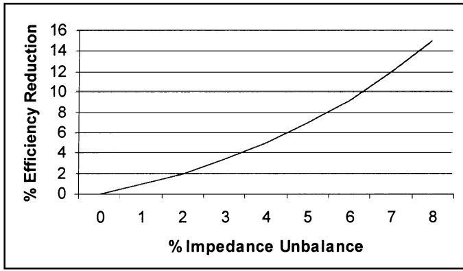
Figure 3: Efficiency Reduction Due to Impedance Unbalance
