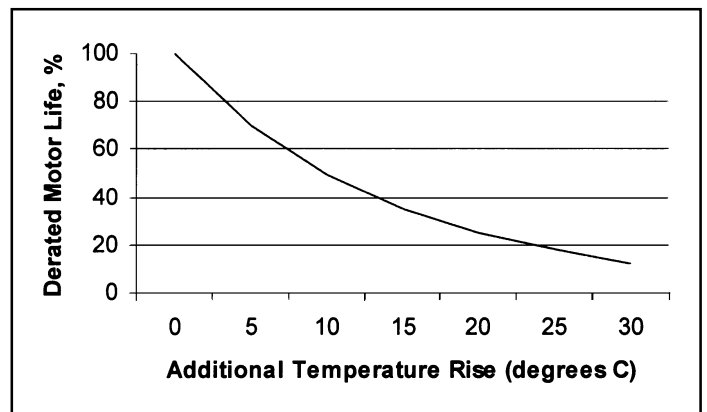
Figure 10: Reduced Motor Life Due to Increased Operating Temperature
