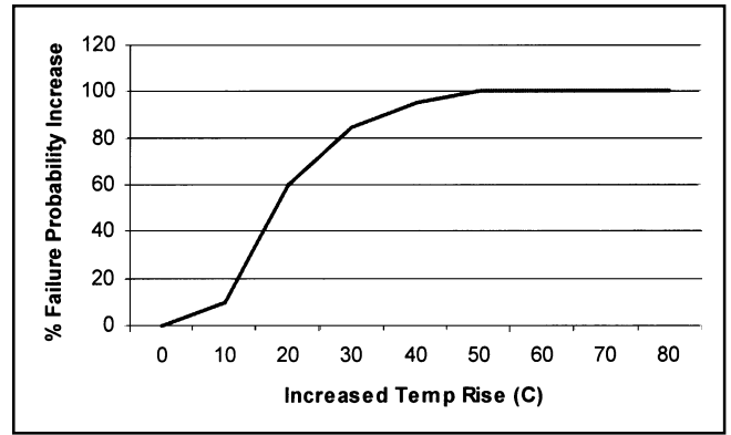
Figure 8: Probability of Failure
