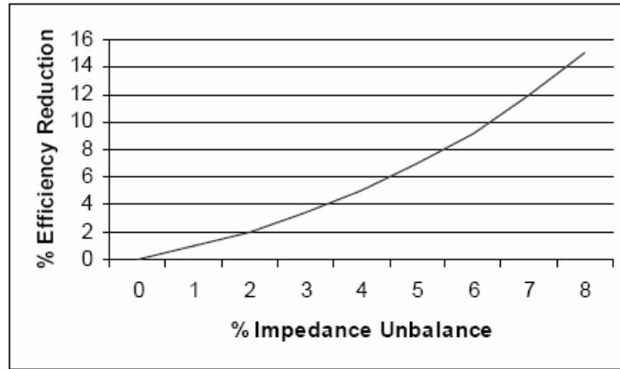
Figure 1: Efficiency Reduction Due to Impedance Unbalance
